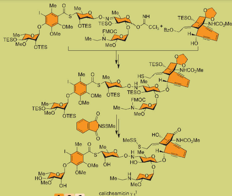
Calicheamicin \gamma_1^1
